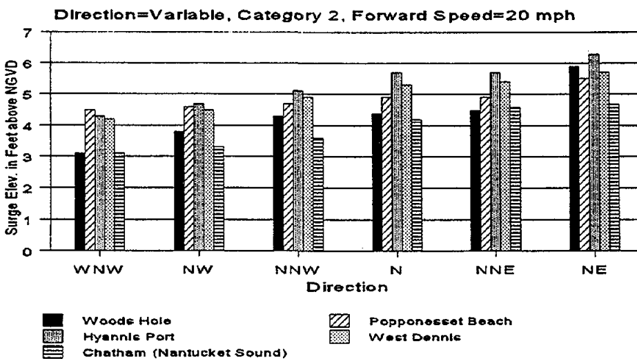
Figure 2.9 Influence of Hurricane Category, Forward Speed and Direction on Surge Heights - Various Locations along the South Shore of Cape Cod.
