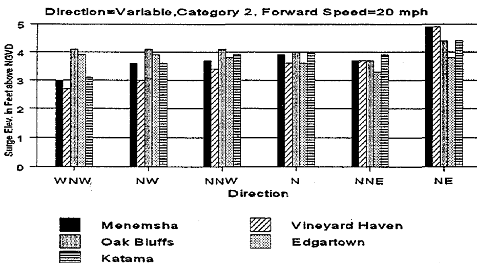
Figure 2.7 Influence of Hurricane Category, Forward Speed and Direction on Surge Heights - Various Locations on Martha's Vineyard.
