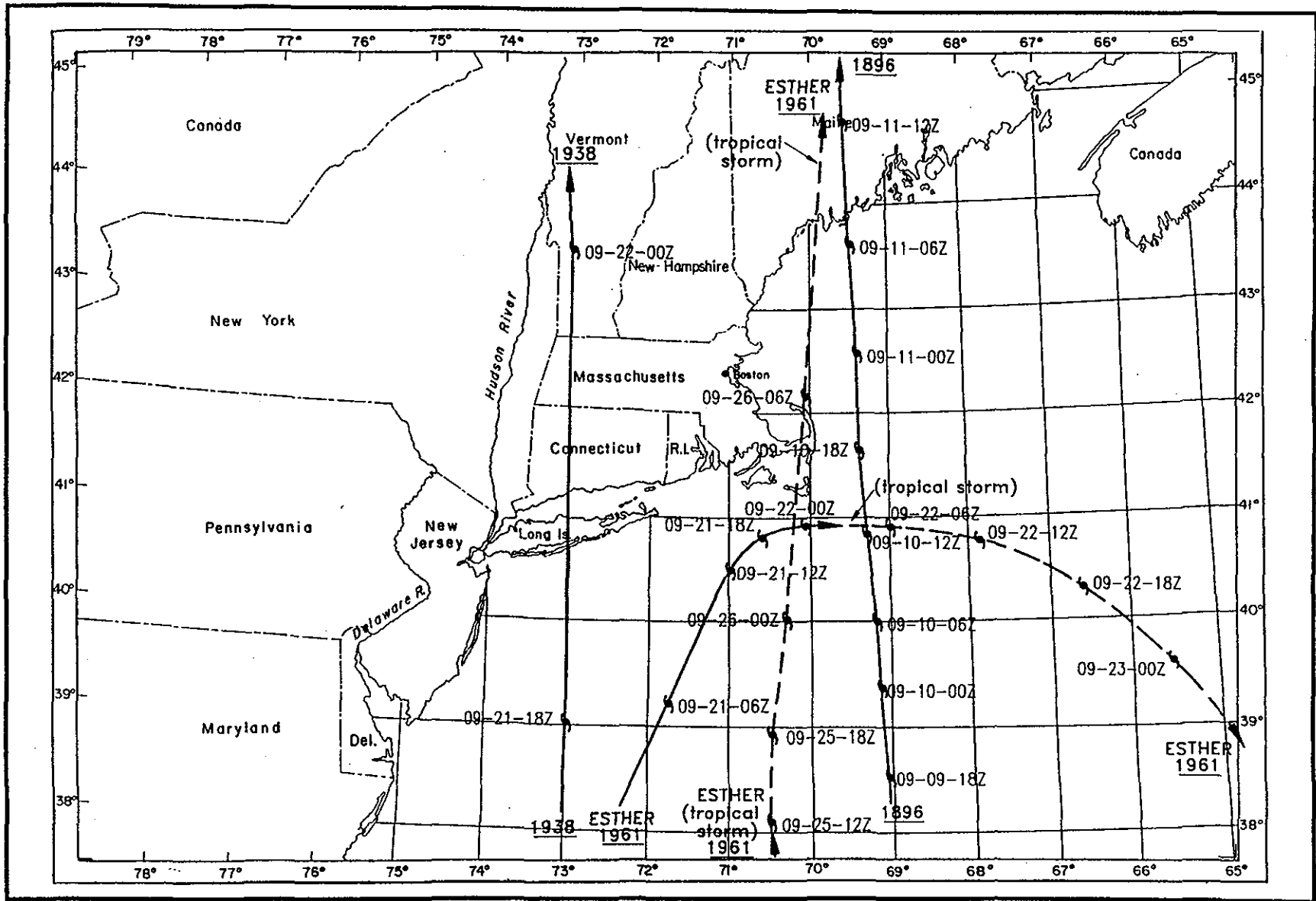
Figure 1.3 Northbound hurricanes and tropical storms passing within 125 statute miles of Boston, Massachusetts from 1886-1996. Source: NHC
