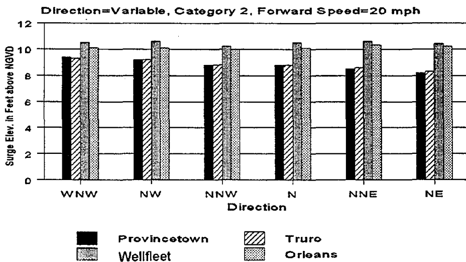
Figure 2.11 Influence of Hurricane Category, Forward Speed and Direction on Surge Heights - Various Locations along the Cape Cod Bay Shore of the Outer Cape.
