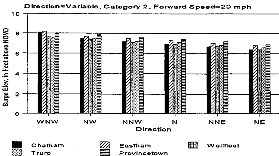
Figure 2.10 Influence of Hurricane Category, Forward Speed and Direction on Surge Heights - Various Locations along the East Shore of Cape Cod.
