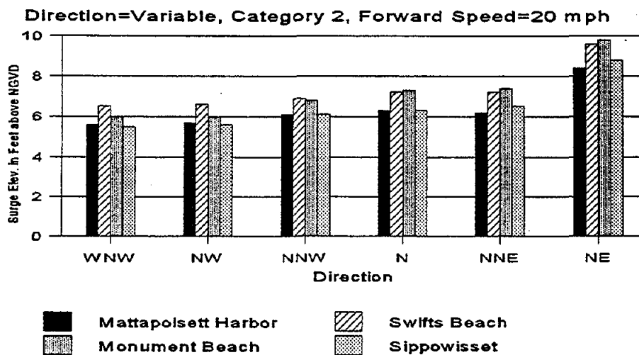
Figure 2.6 Influence of Hurricane Category, Forward Speed and Direction on Surge Heights - Various Locations in Buzzards Bay.
