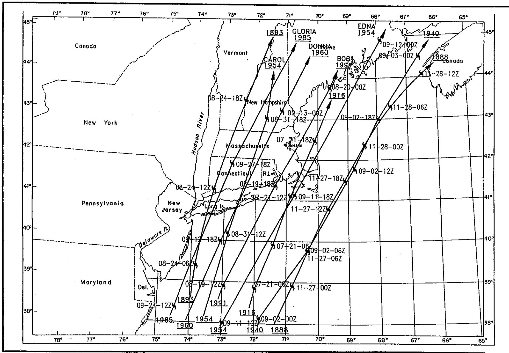
Figure 1.4 North-northeast moving hurricanes and tropical storms passing within 125 statute miles of Boston, Massachusetts from 1886-1996. Source: NHC
