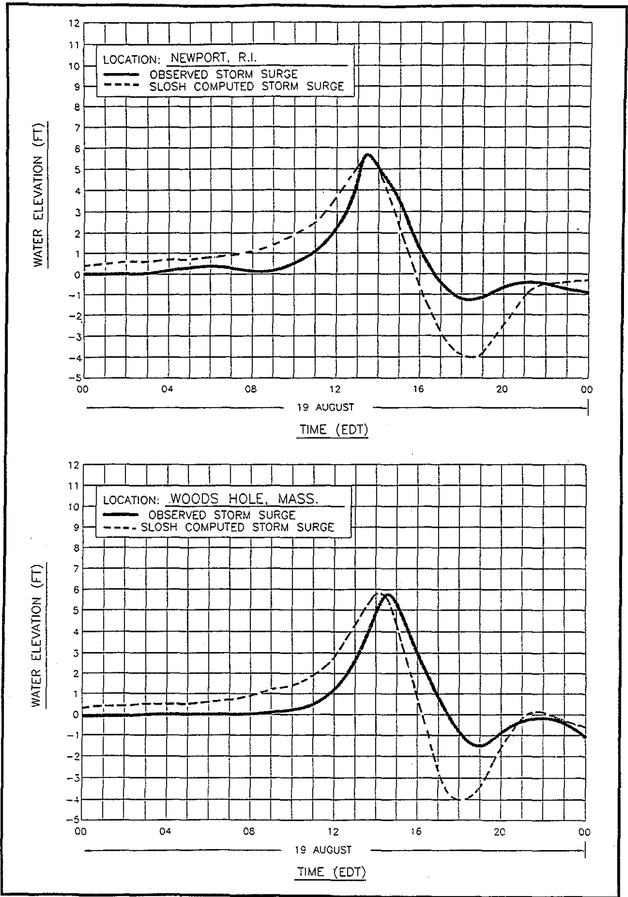
Figure 2.3 SLOSH Model Surge vs. Observed Surge at Newport, RI and Woods Hole, MA, Hurricane Bob, 1991.
