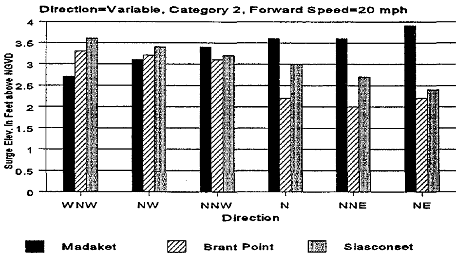
Figure 2.8 Influence of Hurricane Category, Forward Speed, and Direction on Surge Heights - Various Locations on Nantucket.
