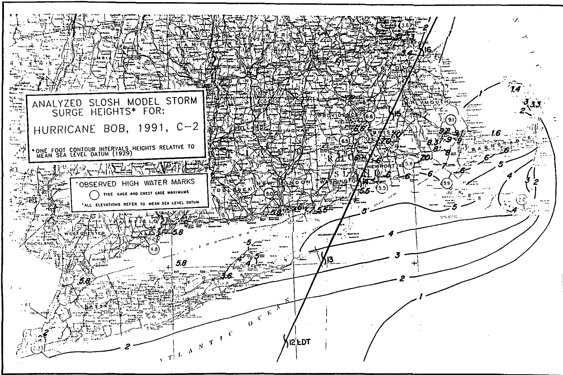
Figure 2.2 SLOSH Model Surge Heights vs. Observed Surge Heights, Hurricane Bob, 1991.
