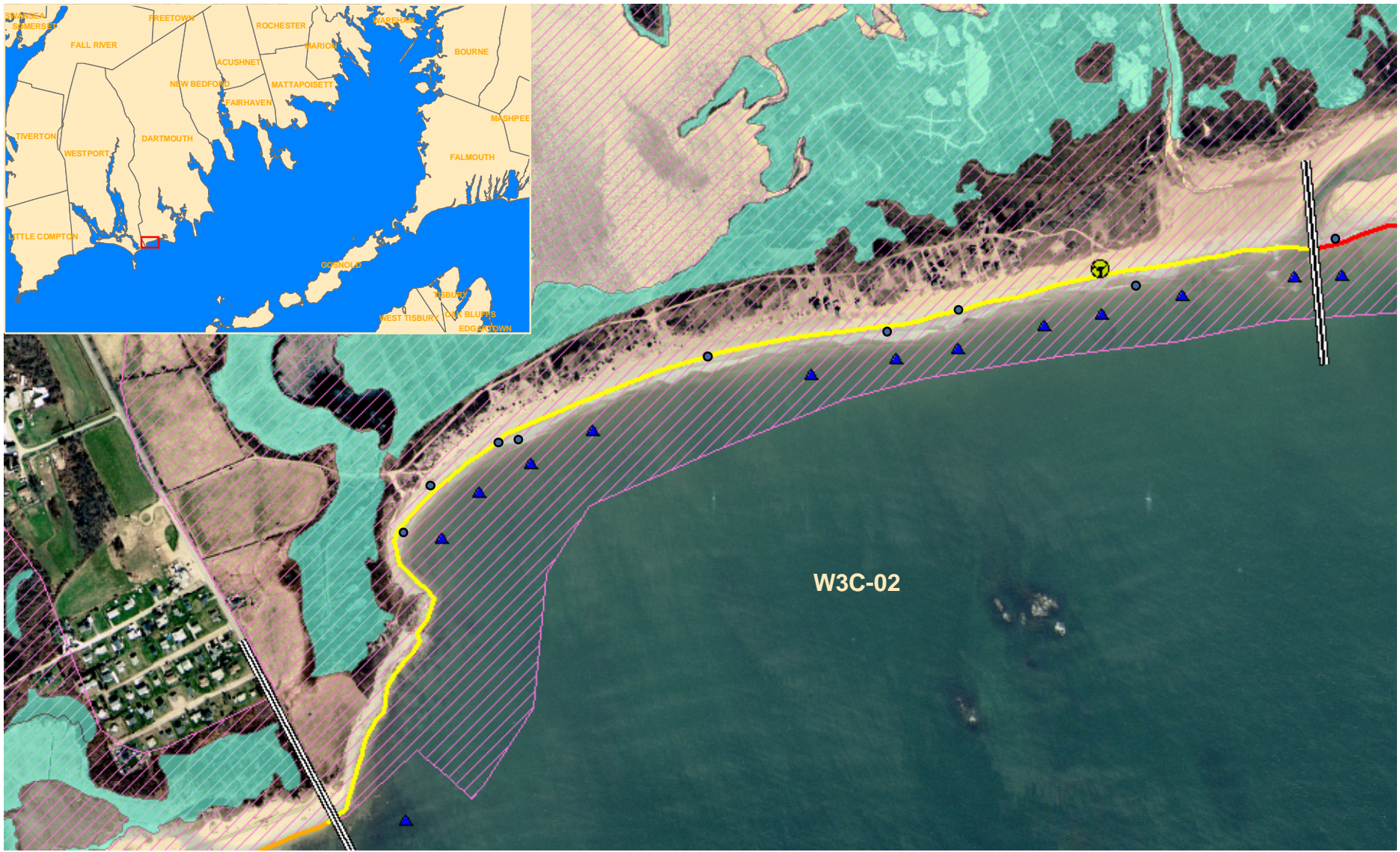
ENTRIX Figure 14 Little Beach W3C-02 Shoreline Segment Summary Bouchard B No. 120 Oil Spill Buzzards Bay, MA
