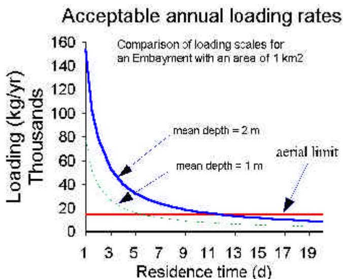
Figure 4. Comparison of aerial limit to volumetric limit in a hypothetical embayment.
