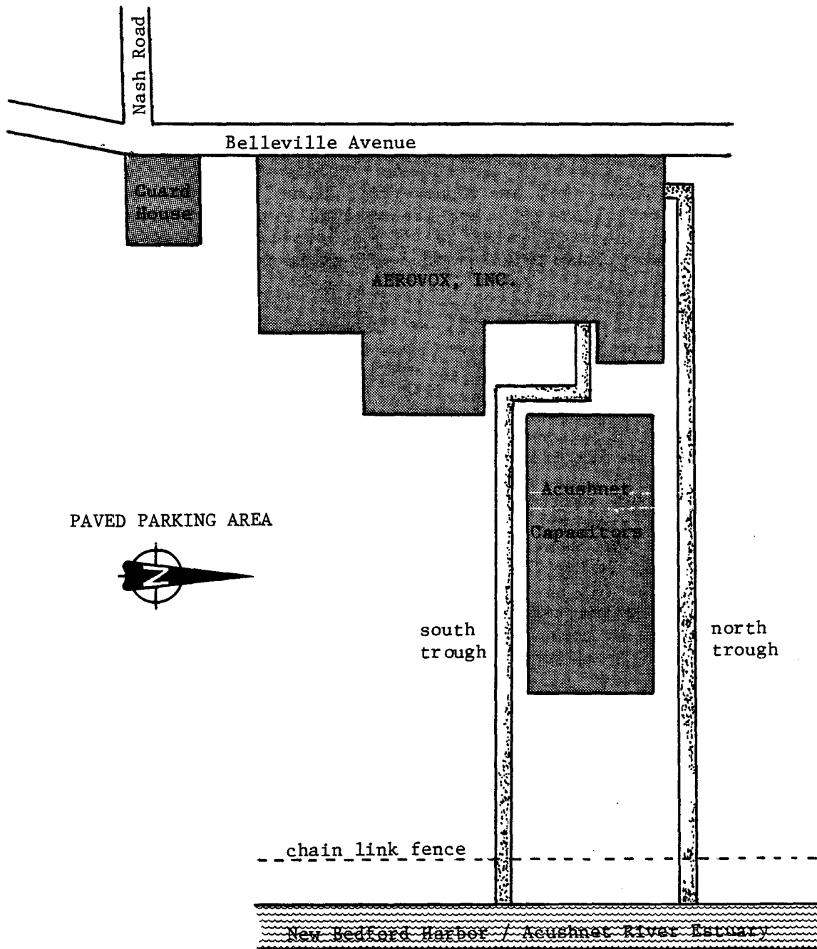
Figure 8. Schematic of Aerovox Incorporated; New Bedford, Massachusetts. figure from: Versar (52), page 3.
