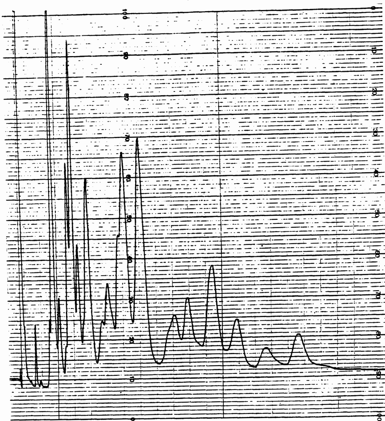
Figure 2. Chromatogram of a One Hour Ambient Air Sample Taken at the New Bedford Municipal Landfill. from: Stratton, et al. (9), page 30.
