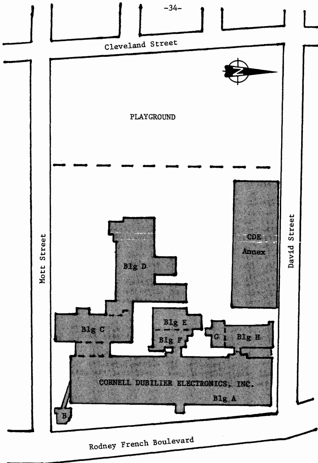
Cornell Dubilier Electronics Incorporated plant layout. figure from EG&G (55), page 2.
