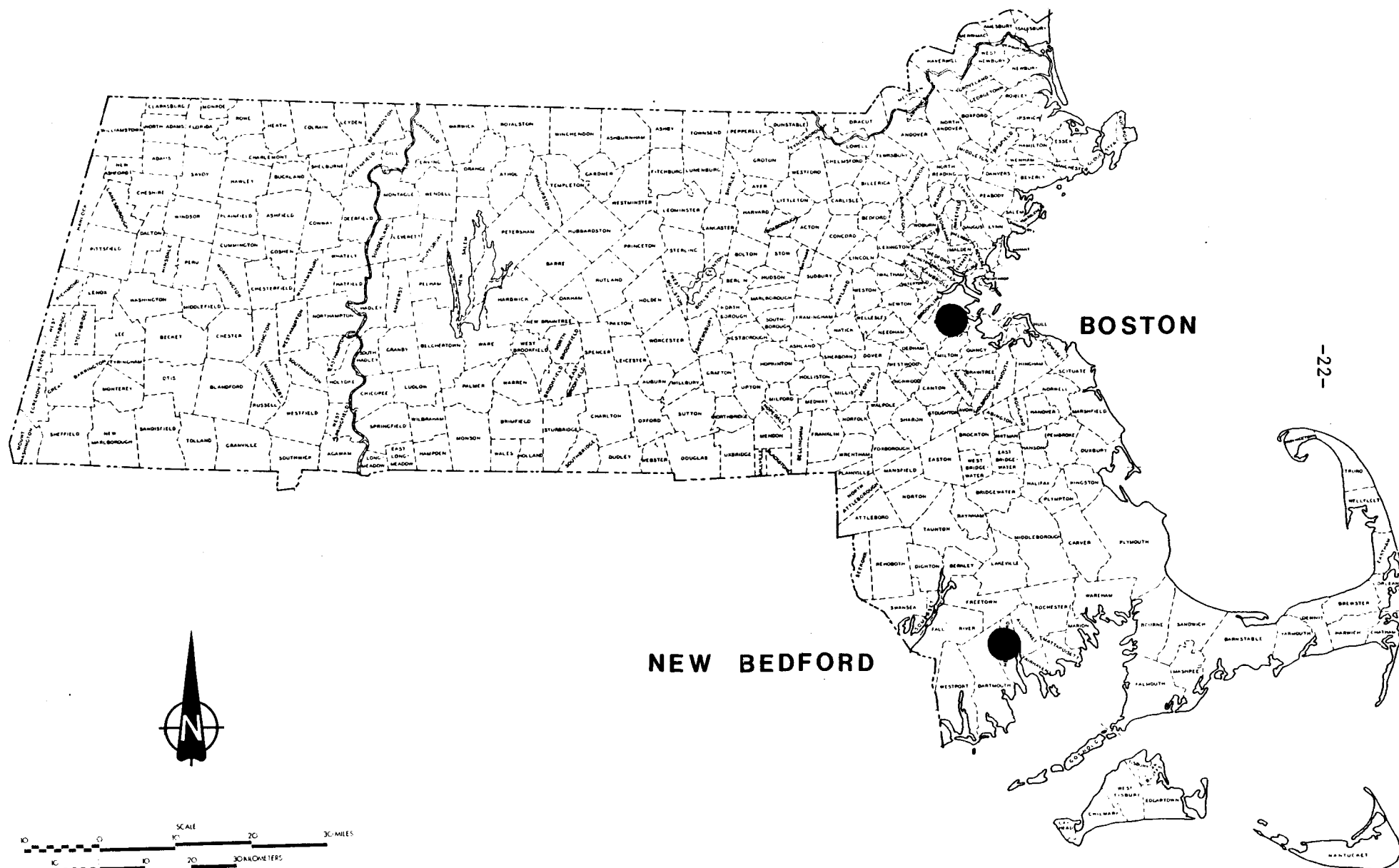
Figure 5. Locational Map
