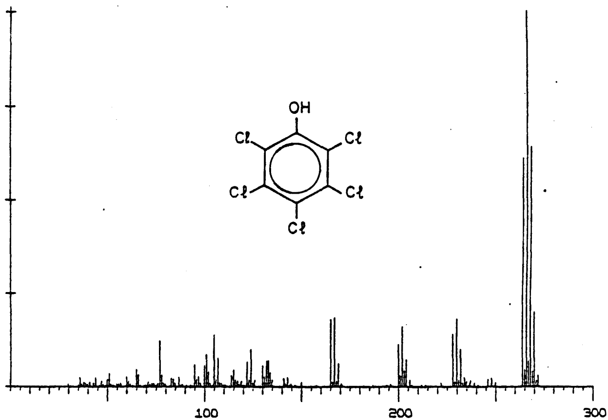
Figure 4. Gas Chromatograph / Mass Spectrophotometer Analysis of Pentachlorophenol. from: Biemann (10).
