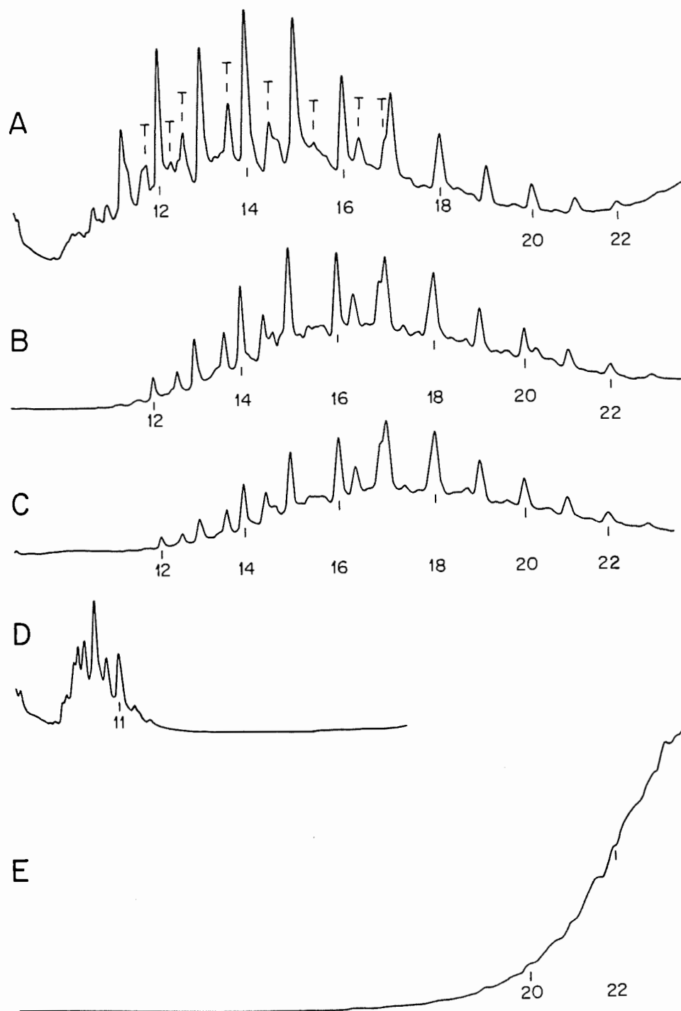
Figure 3. Gas Chromatograms. Top to bottom: A: #2 Fuel oil. B: Sediments in Wild Harbor Basin, 12 days after accident. C: Oil recovered from water in Wild Harbor Basin, 2 months after accident. D: 2-cycle outboard motor oil. E: SAE #10 Lubricating oil. T marks position of isoprenoid alkanes.
