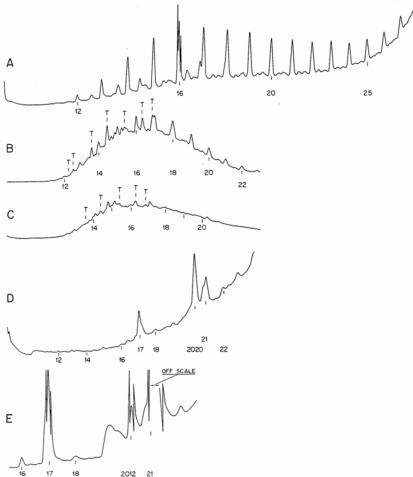
Figure 4. Gas chromatograms. Top to bottom: A: Tar balls, n-hexadecane added as standard. B: Oysters, Wild Harbor River. C: Scallops, West Falmouth Harbor. D: Oysters, Waquoit Bay. E: Rhizosolenia setigera . Chromatograms 4A, 4 D-E at different column lengths or program rates. T marks position of isoprenoid alkanes.
